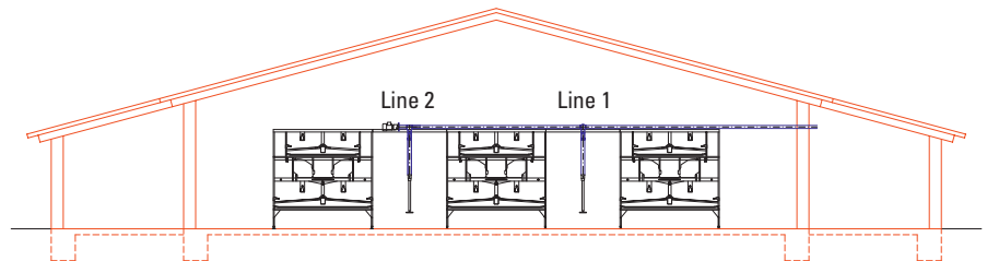
Cross section of the house: PickPuck with automatic filling
